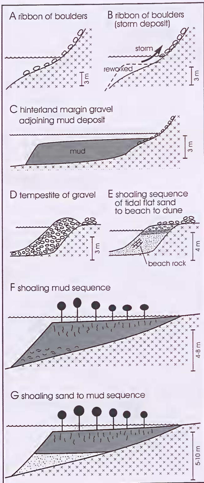
Figure 6. A selection of stratigraphic packages from accretionary systems in the Kimberley region showing their lithologic sequence.
